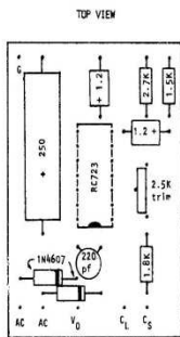
REGULATOR BOARD COMPONENT LAYOUT
